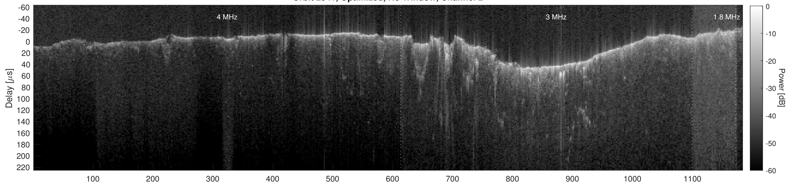
Orbit 2941, Cluttergram
