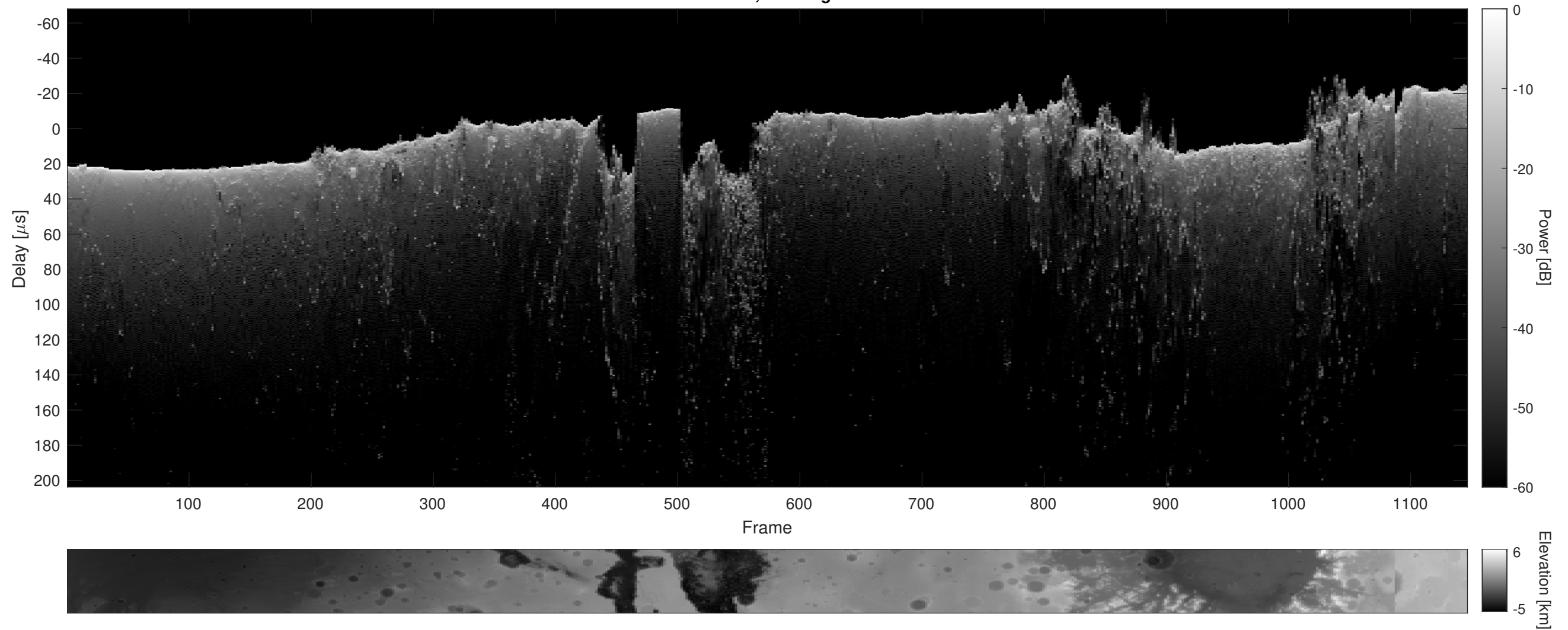
Orbit 2942, Cluttergram
