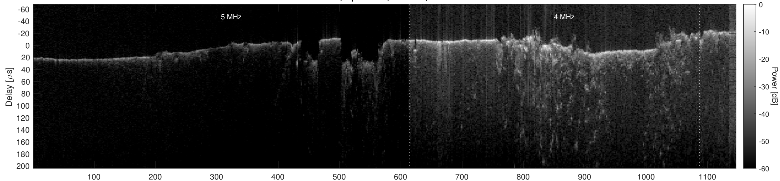
Orbit 2942, Optimized, Window, Channel 2
