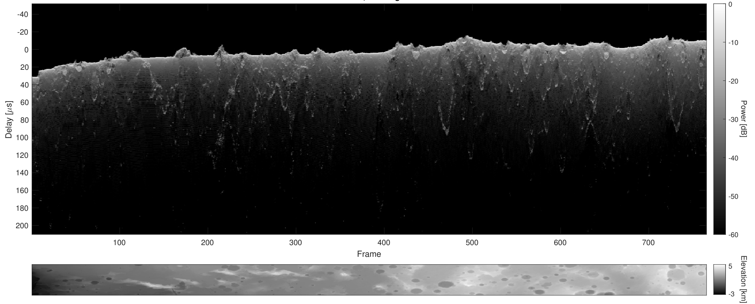
Orbit 2943, Cluttergram
