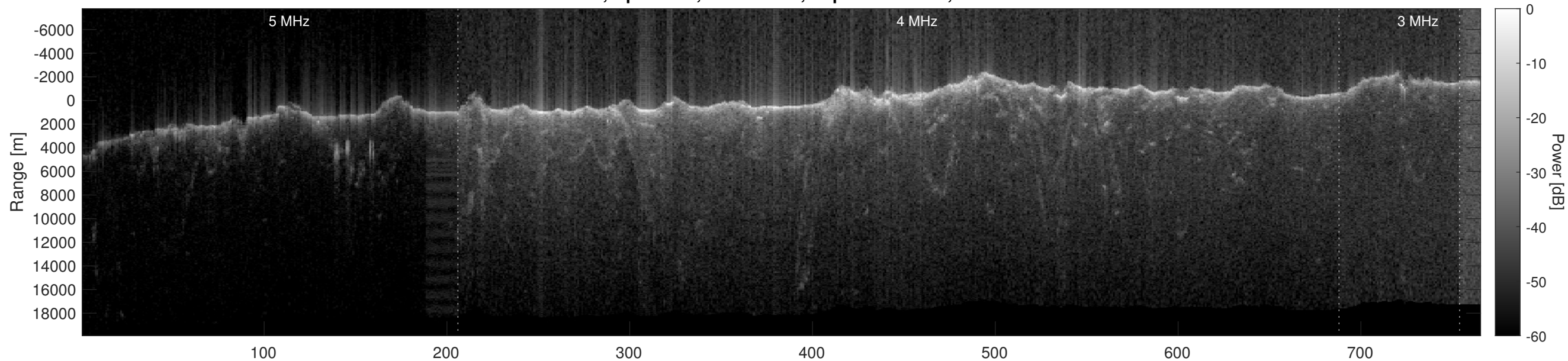
Orbit 2943, Optimized, No Window, Depth-Corrected, Channel 2
