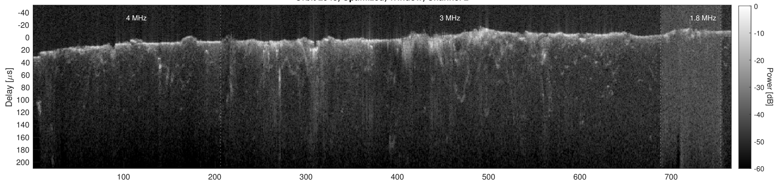
Orbit 2943, Cluttergram
