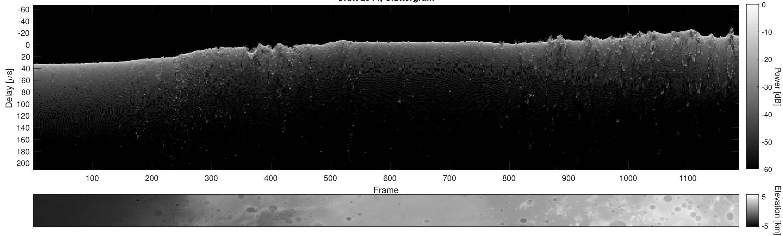
Orbit 2944, Cluttergram
