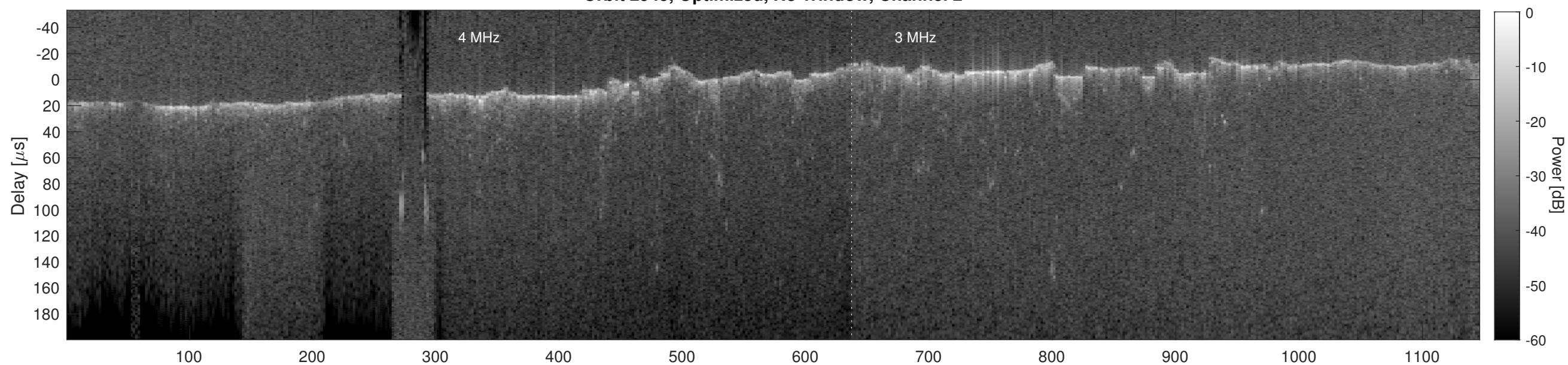
Orbit 2945, Cluttergram
