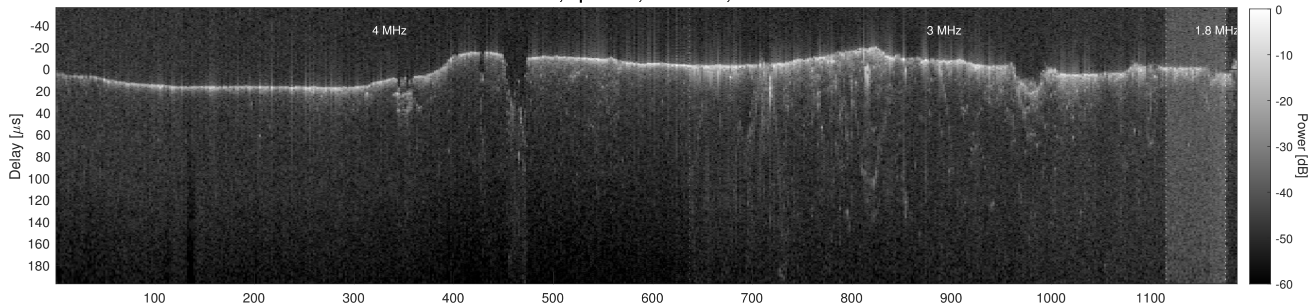
Orbit 2946, Cluttergram
