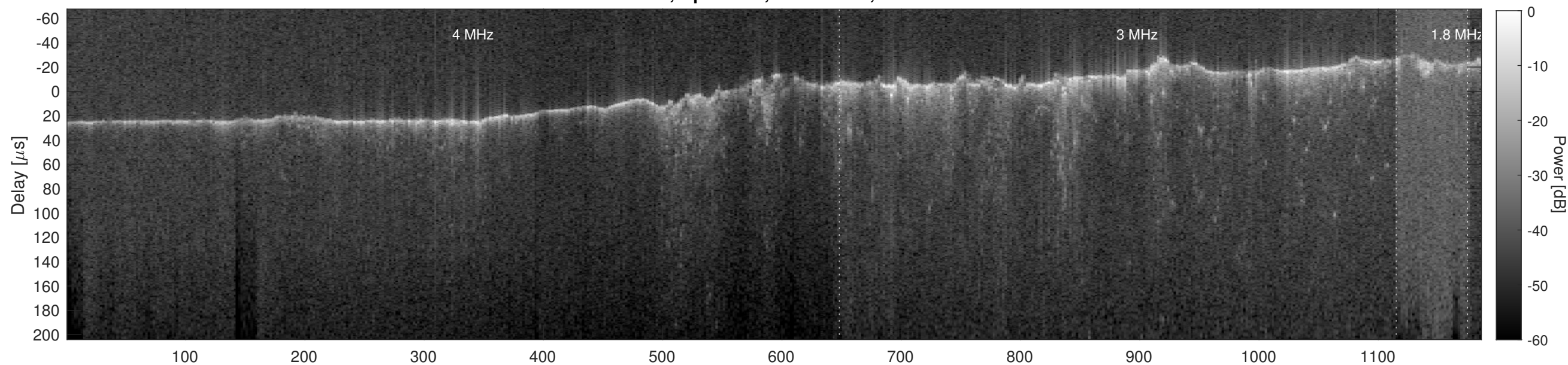
Orbit 2947, Cluttergram
