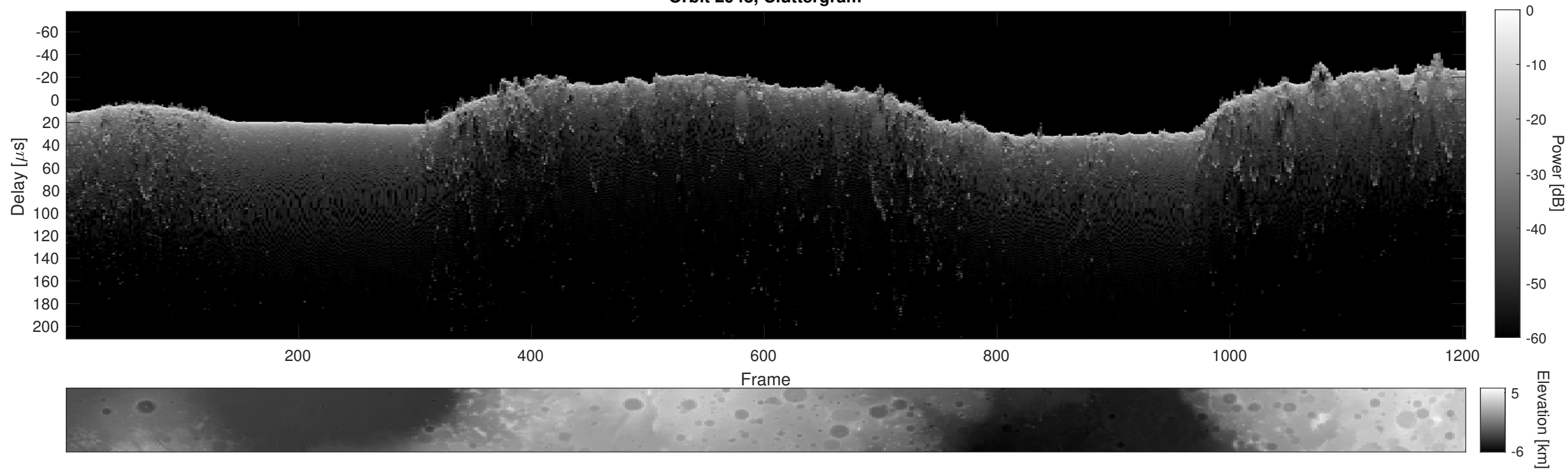
Orbit 2948, Cluttergram
