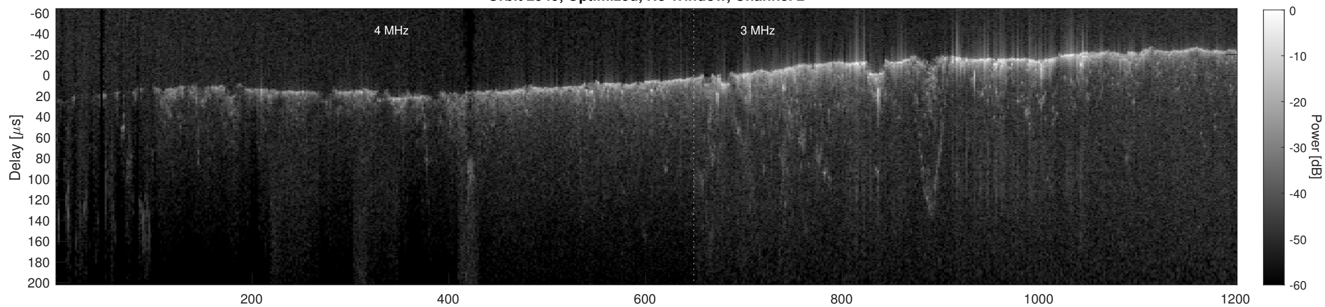
Orbit 2949, Cluttergram
