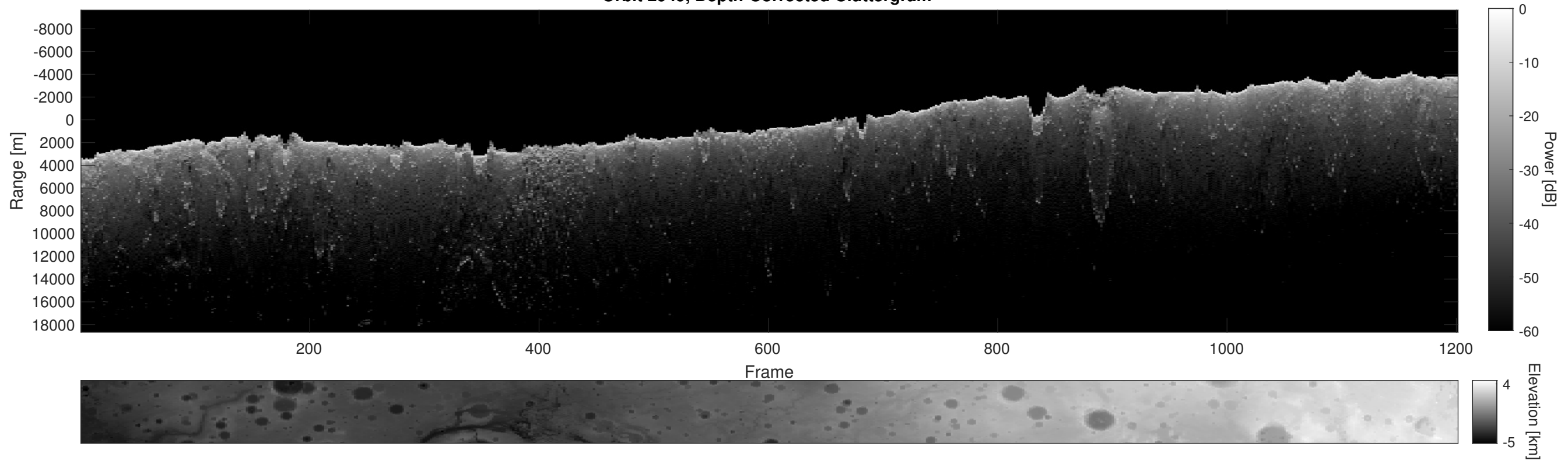
Orbit 2949, Depth-Corrected Cluttergram
