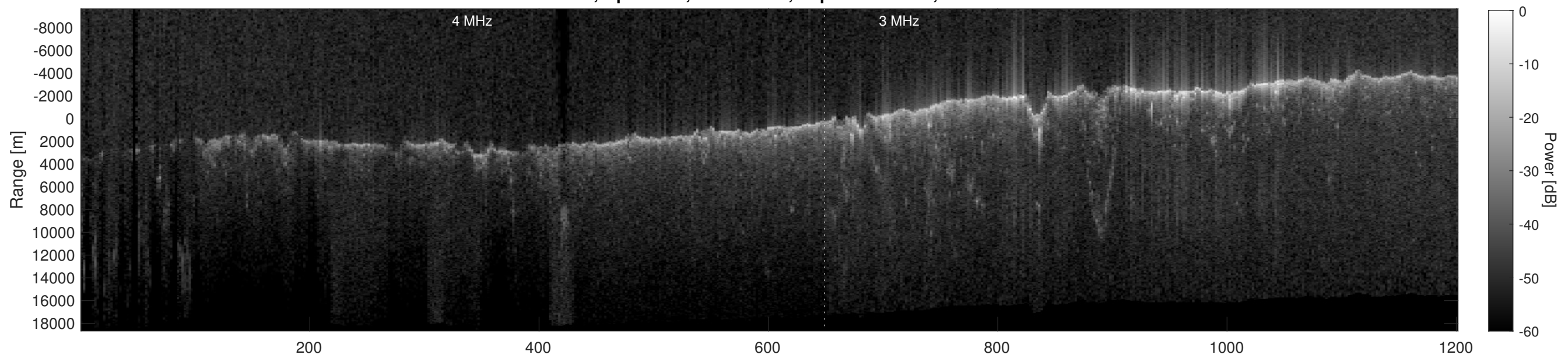
Orbit 2949, Depth-Corrected Cluttergram
