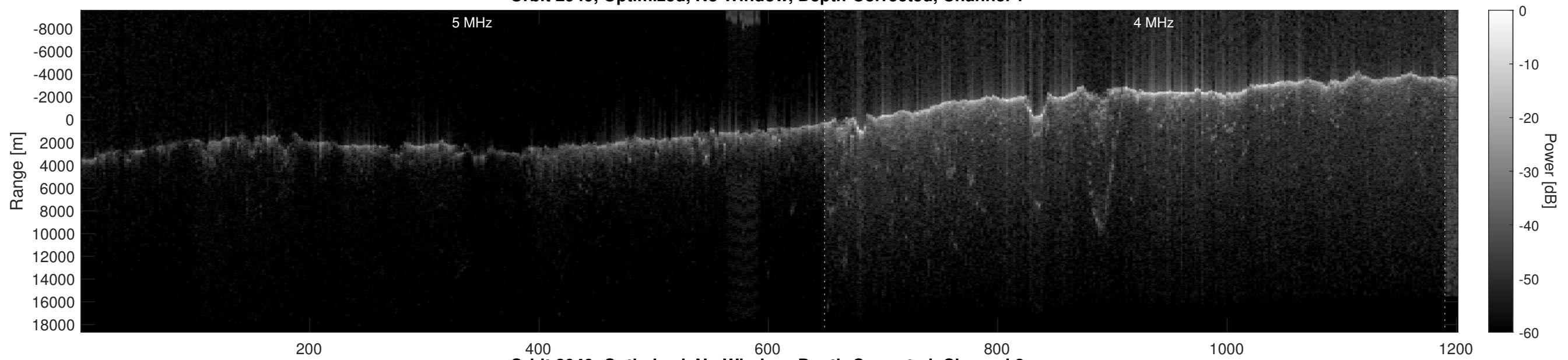
Orbit 2949, Optimized, No Window, Depth-Corrected, Channel 2
