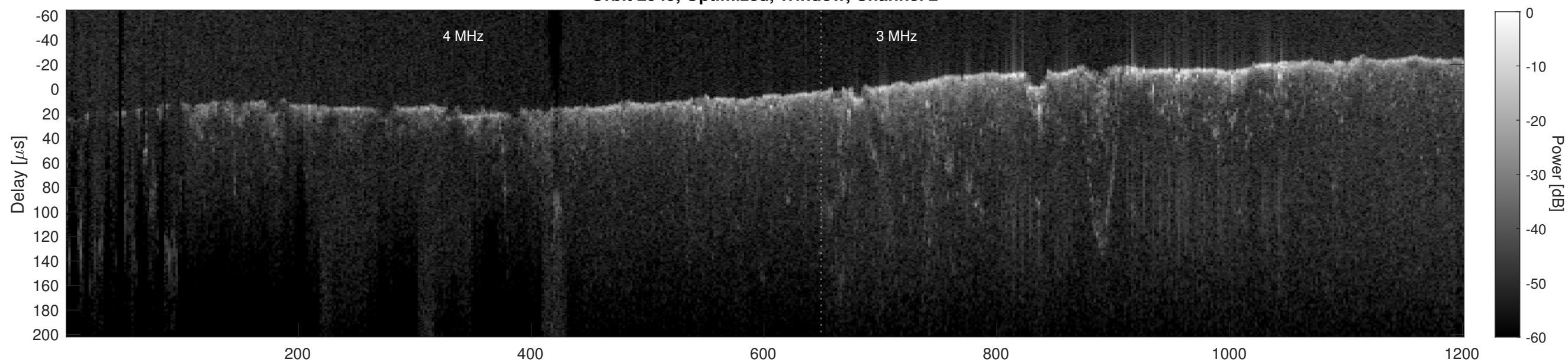
Orbit 2949, Cluttergram
