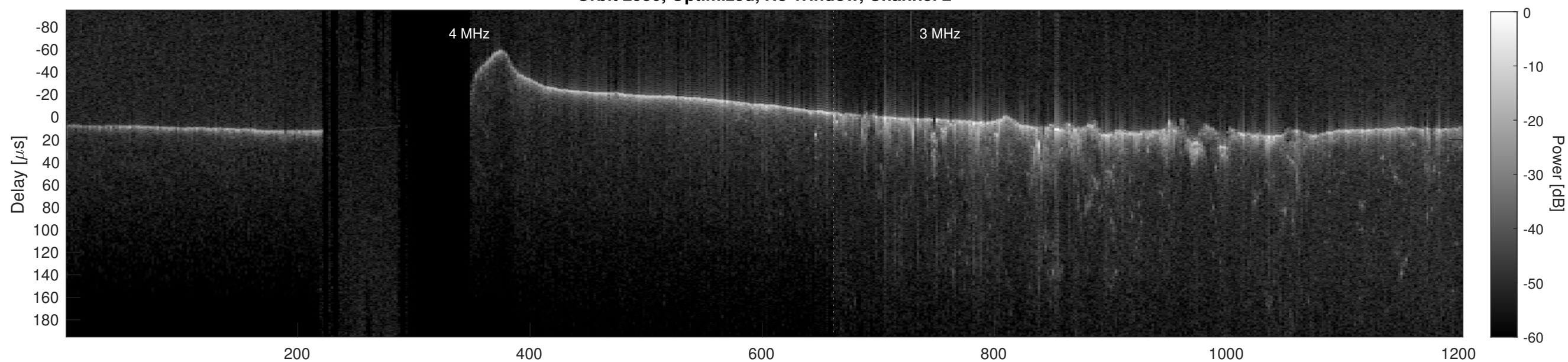
Orbit 2950, Cluttergram
