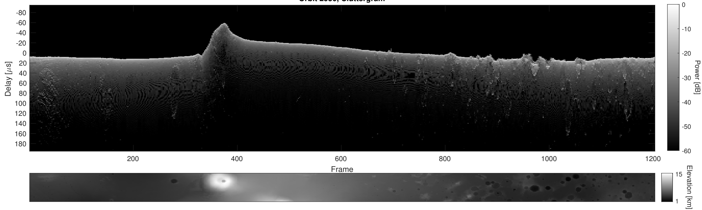
Orbit 2950, Cluttergram
