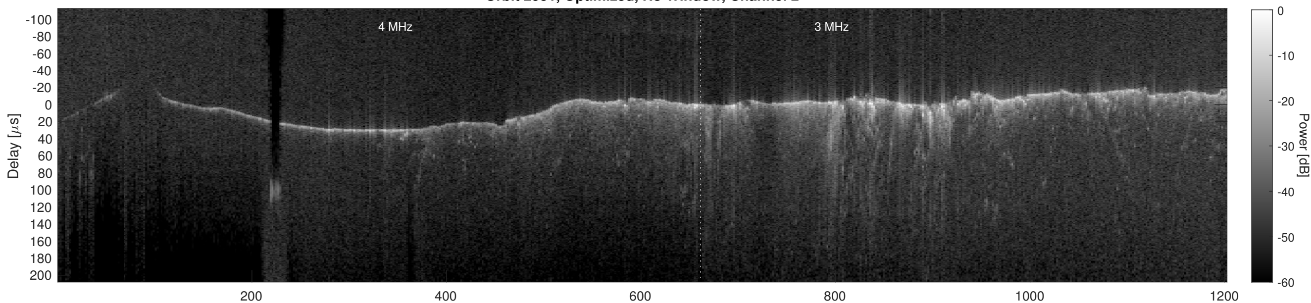
Orbit 2951, Cluttergram
