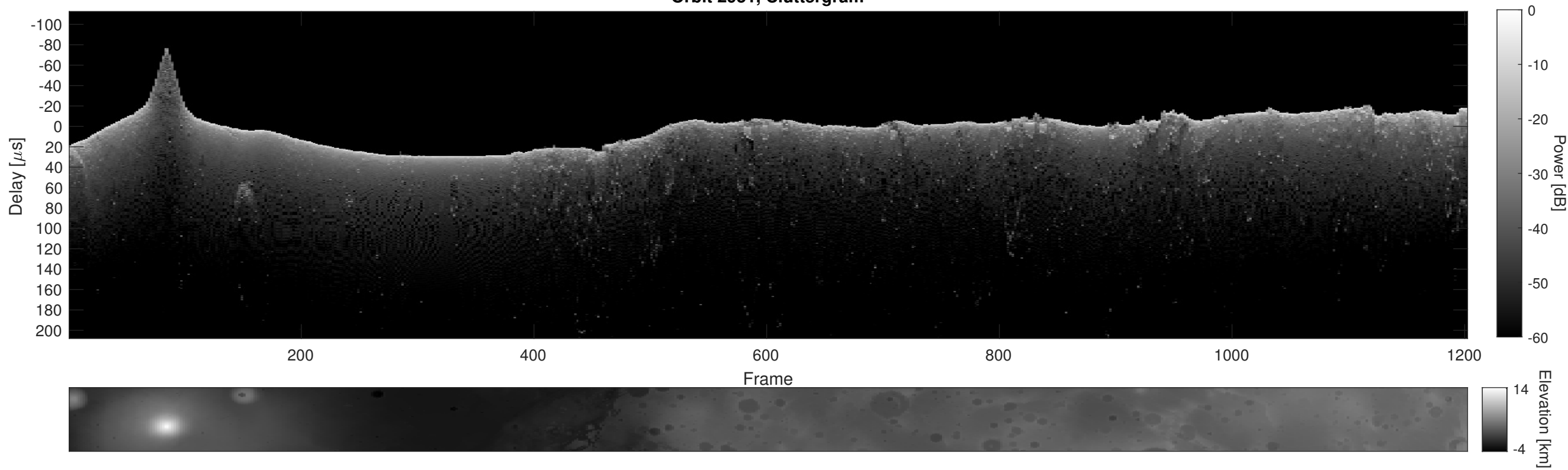
Orbit 2951, Cluttergram
