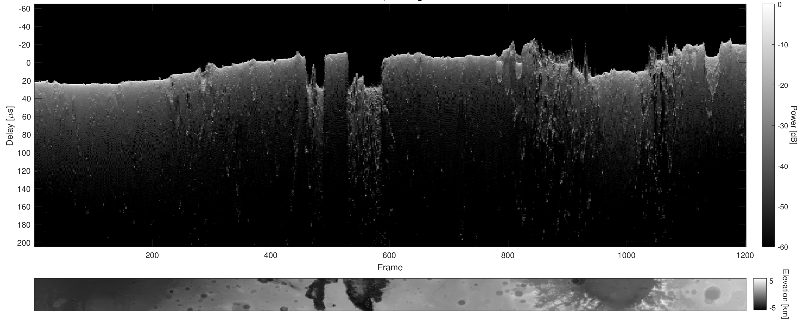
Orbit 2953, Cluttergram
