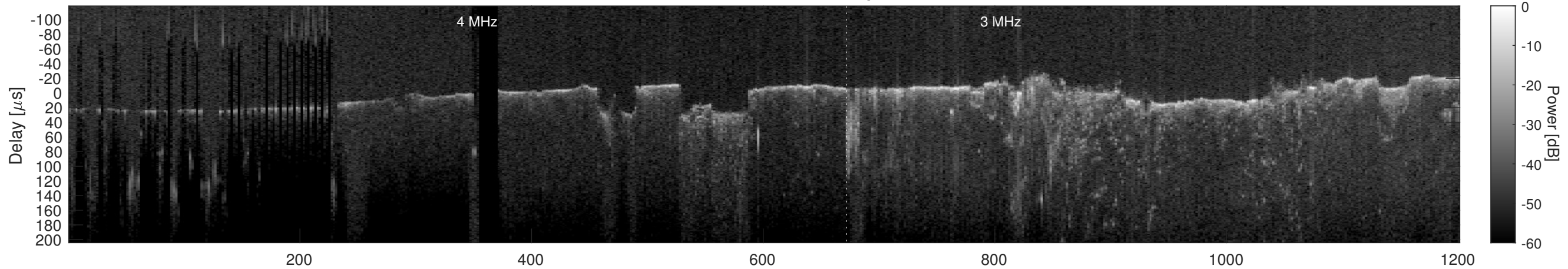
Orbit 2953, Cluttergram
