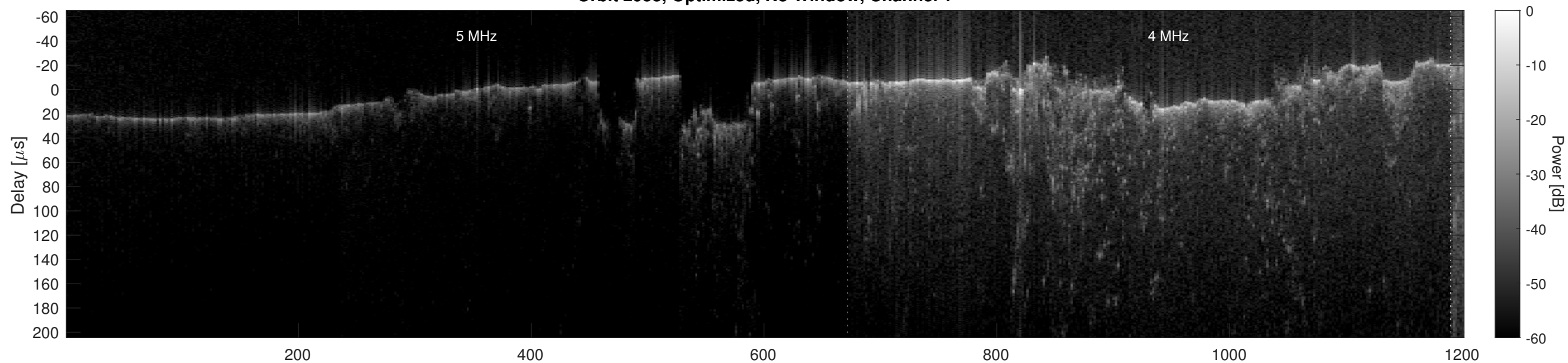
Orbit 2953, Optimized, No Window, Channel 2
