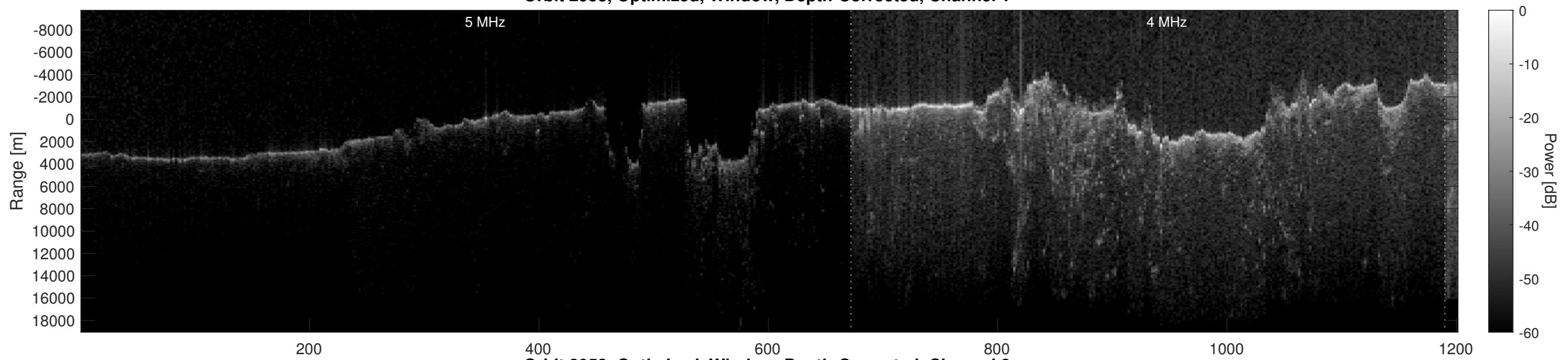
Orbit 2953, Optimized, Window, Depth-Corrected, Channel 2
