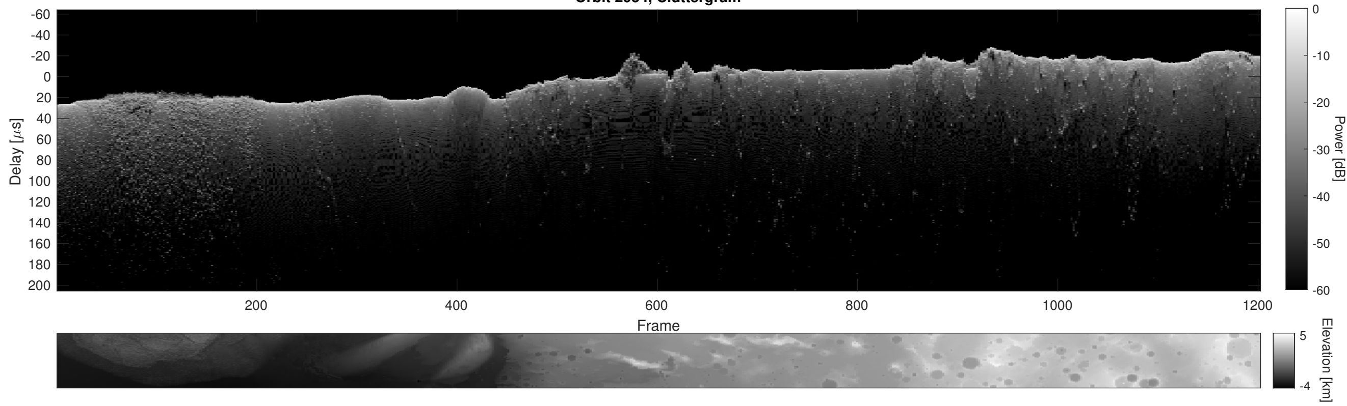
Orbit 2954, Cluttergram
