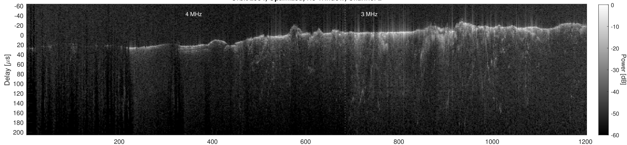
Orbit 2954, Cluttergram
