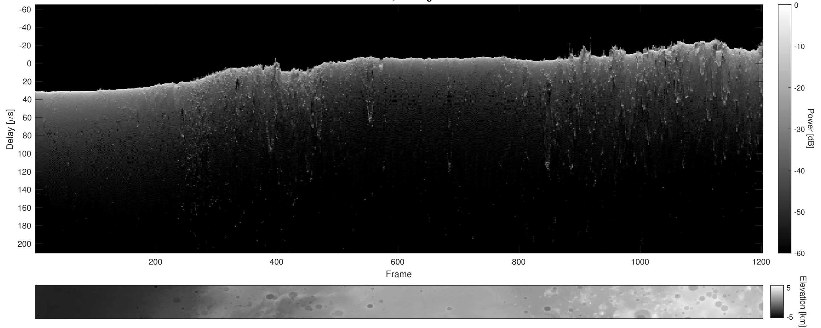
Orbit 2955, Cluttergram
