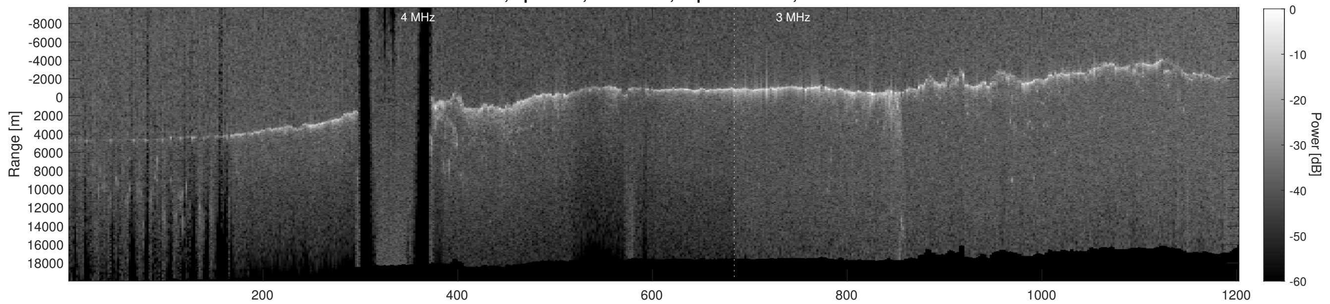
Orbit 2955, Depth-Corrected Cluttergram
