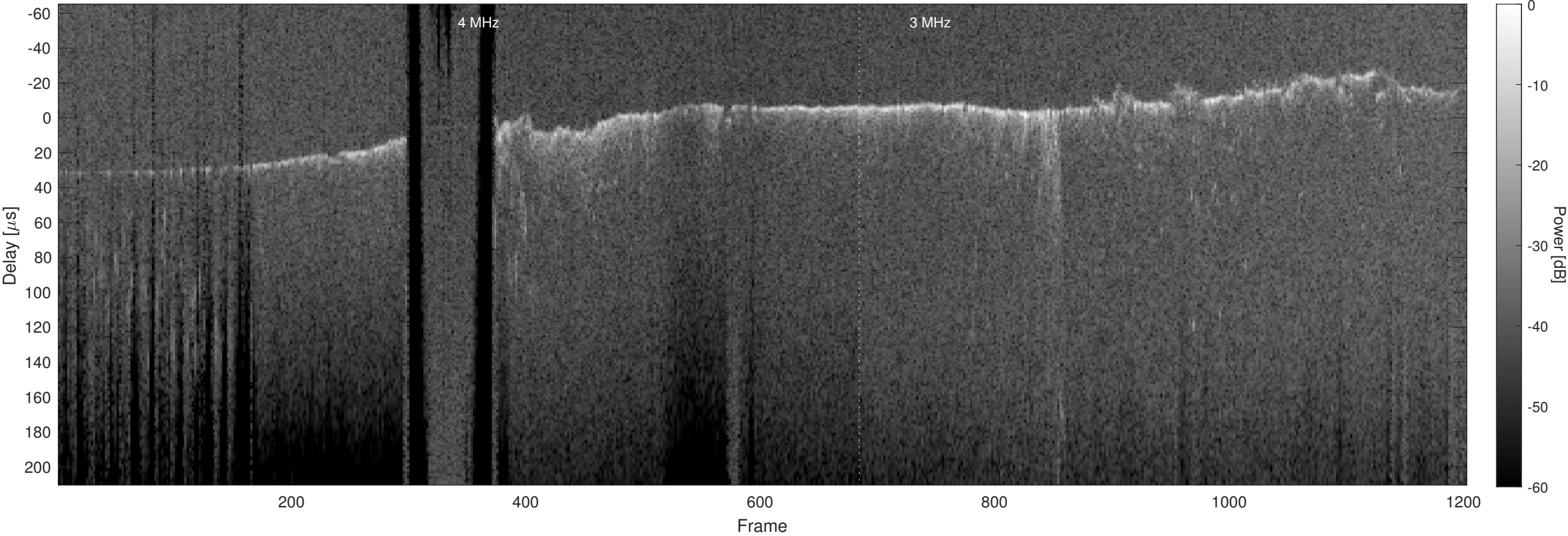
Orbit 2955, Optimized, Window, Channel 2
