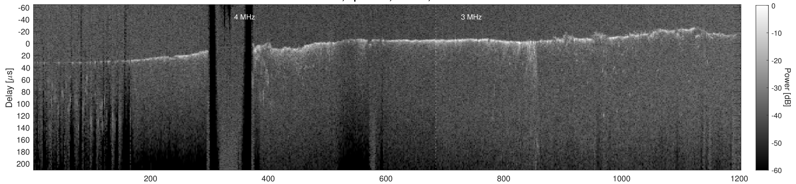
Orbit 2955, Cluttergram
