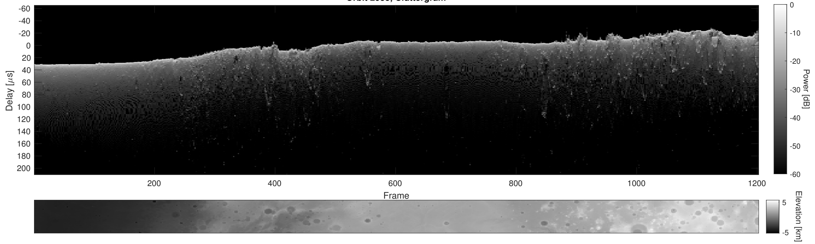
Orbit 2955, Cluttergram
