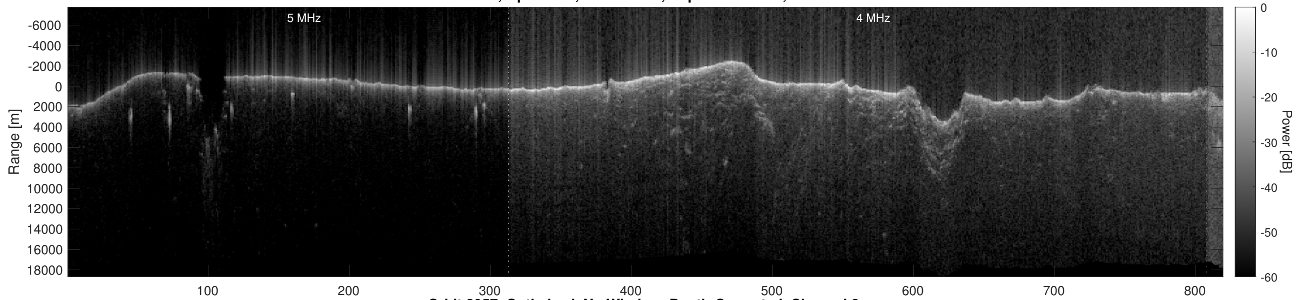
Orbit 2957, Optimized, No Window, Depth-Corrected, Channel 2
