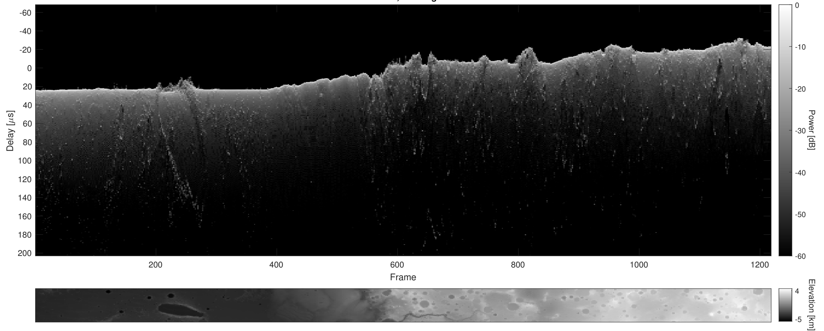
Orbit 2958, Cluttergram
