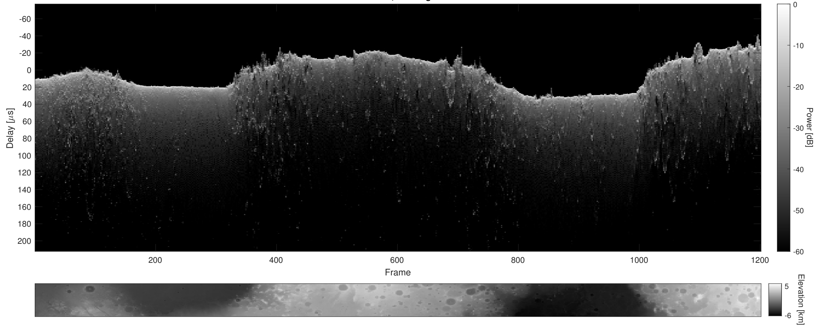
Orbit 2959, Cluttergram
