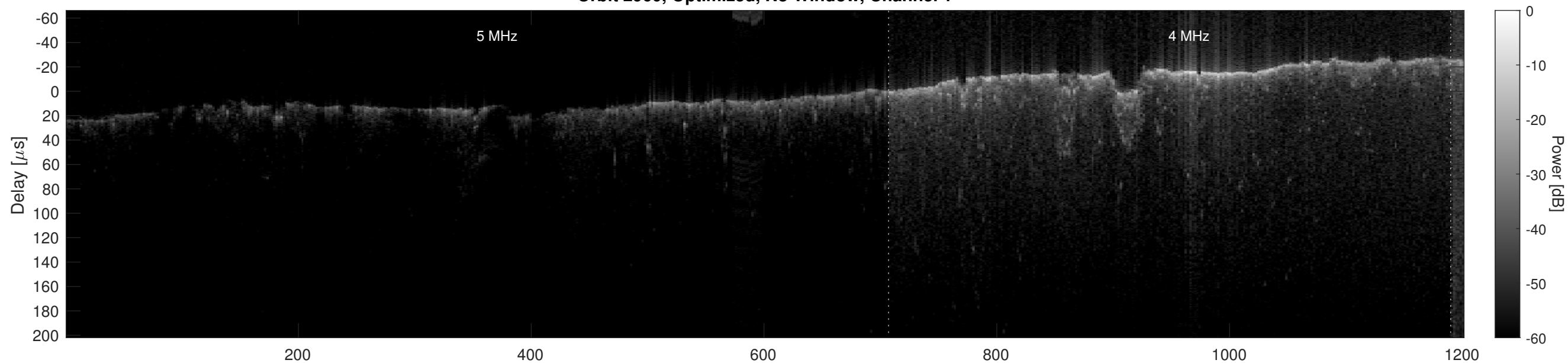
Orbit 2960, Optimized, No Window, Channel 2
