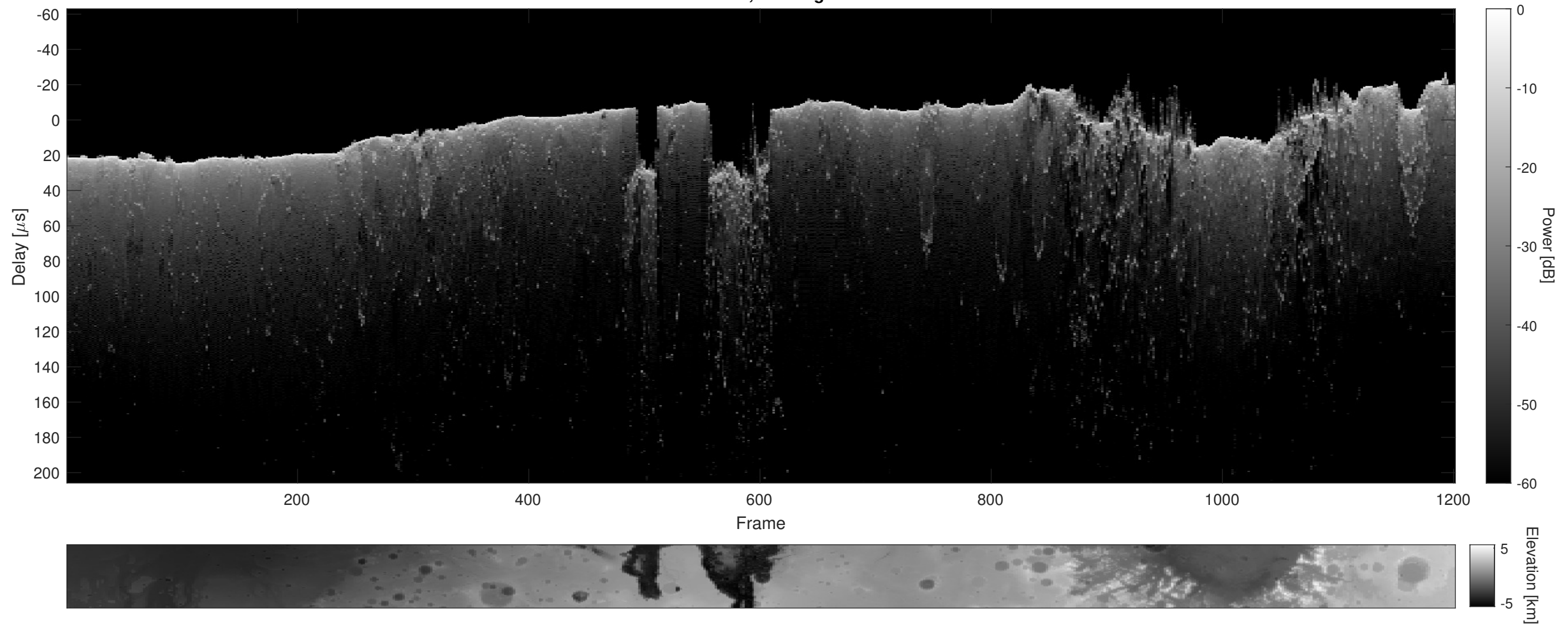
Orbit 2964, Cluttergram
