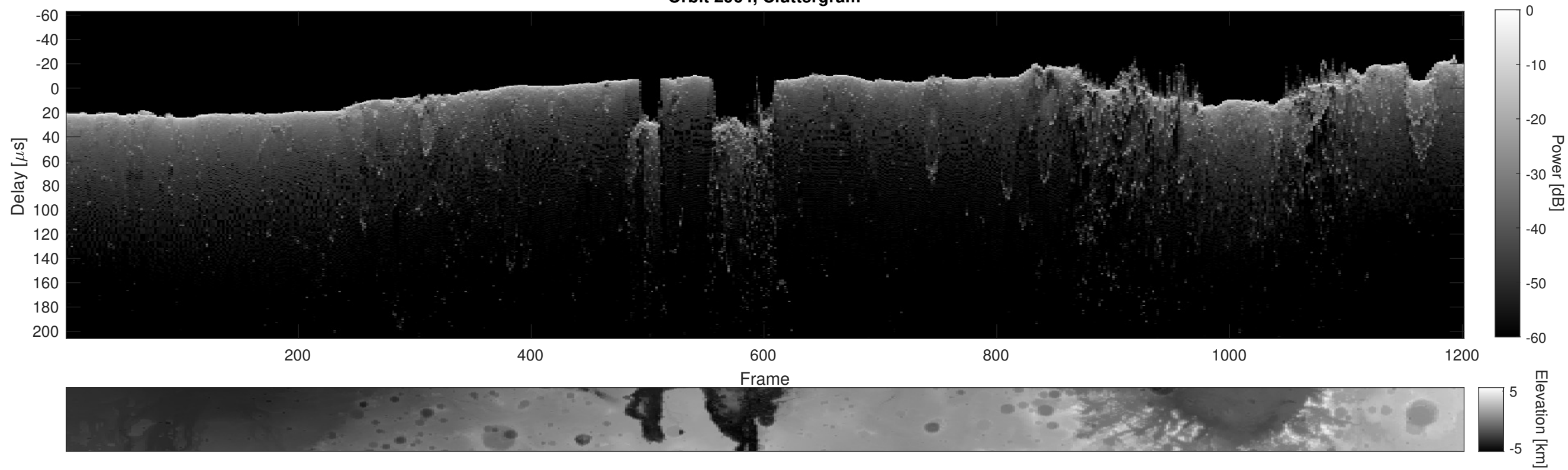
Orbit 2964, Cluttergram
