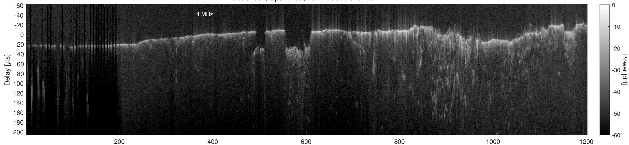
Orbit 2964, Cluttergram
