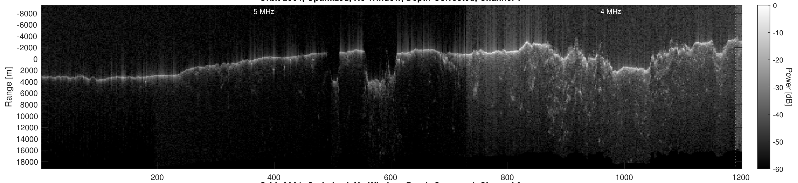
Orbit 2964, Optimized, No Window, Depth-Corrected, Channel 2
