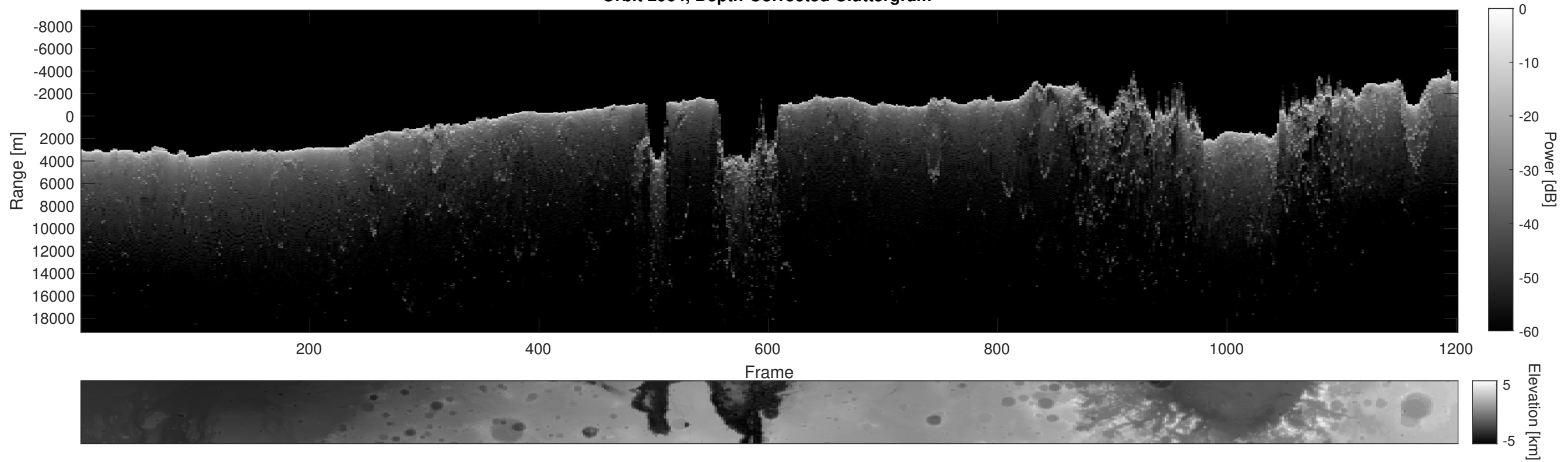
Orbit 2964, Depth-Corrected Cluttergram
