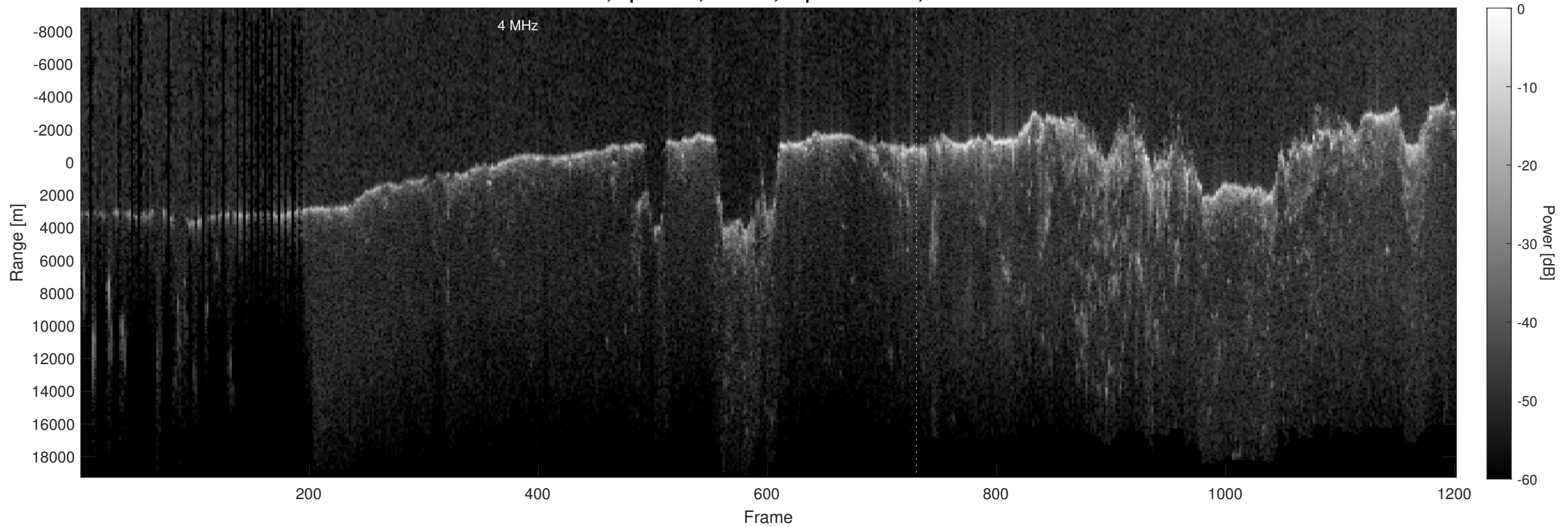
Orbit 2964, Optimized, Window, Depth-Corrected, Channel 2
