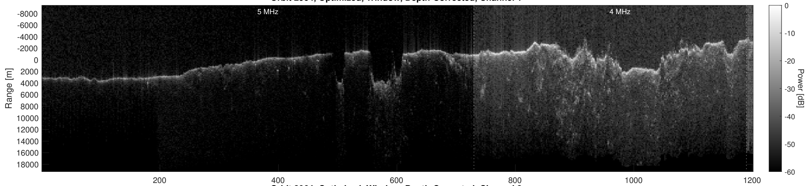
Orbit 2964, Optimized, Window, Depth-Corrected, Channel 2
