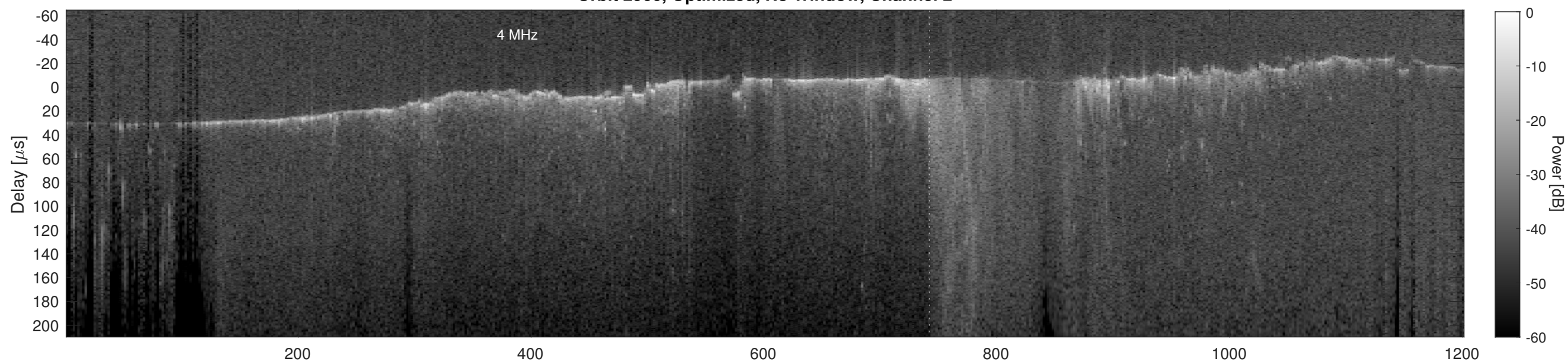
Orbit 2966, Cluttergram
