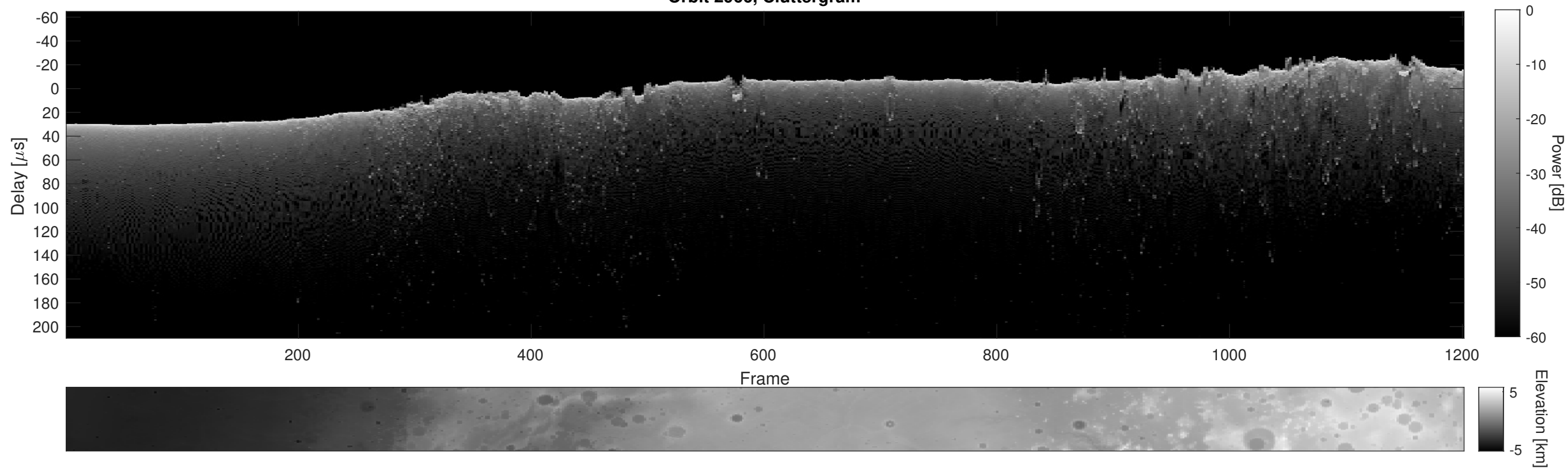
Orbit 2966, Cluttergram
