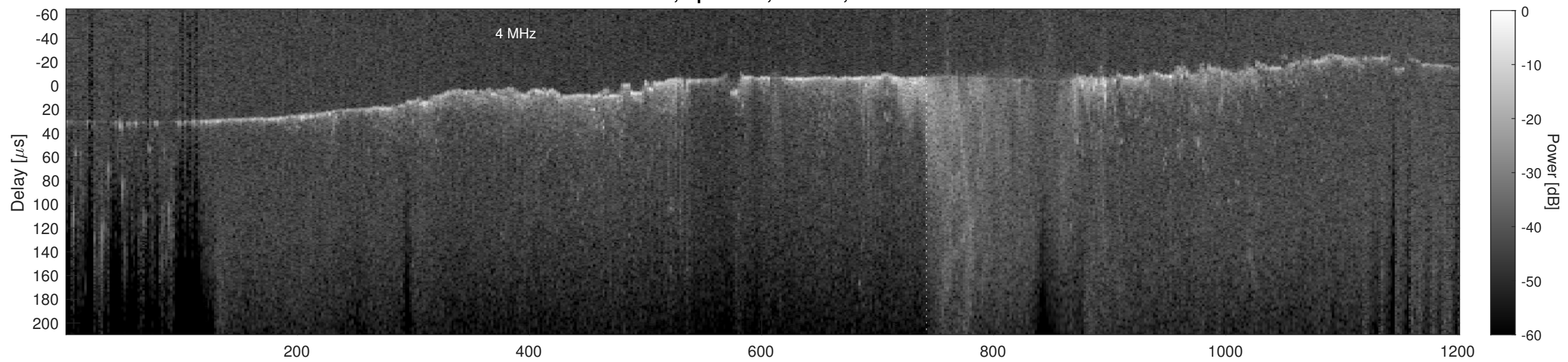
Orbit 2966, Cluttergram
