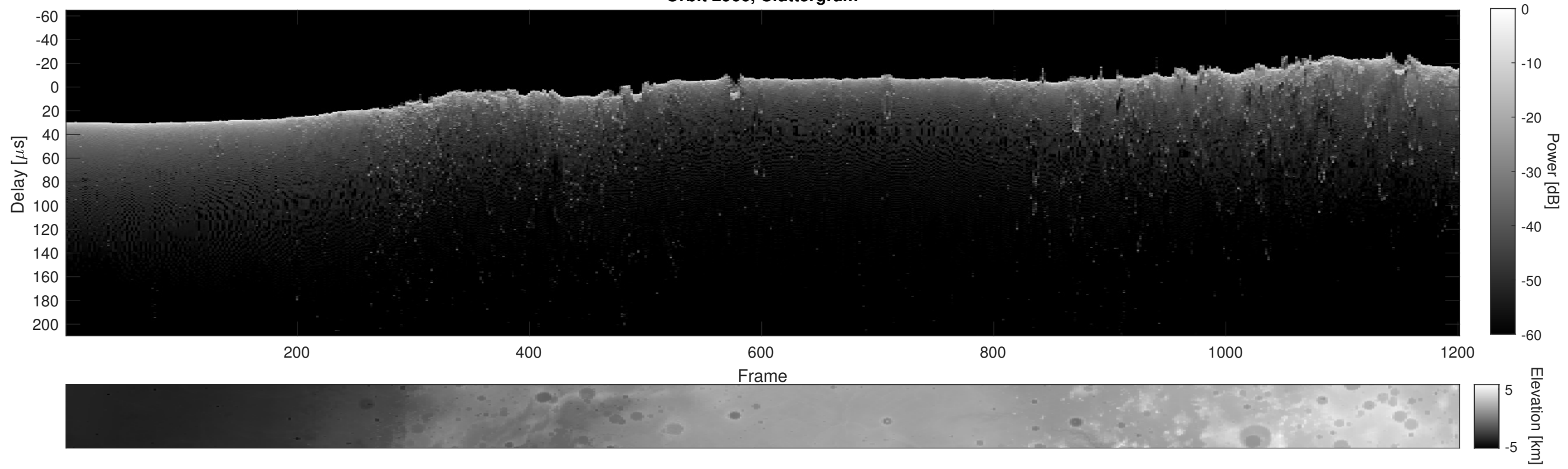
Orbit 2966, Cluttergram
