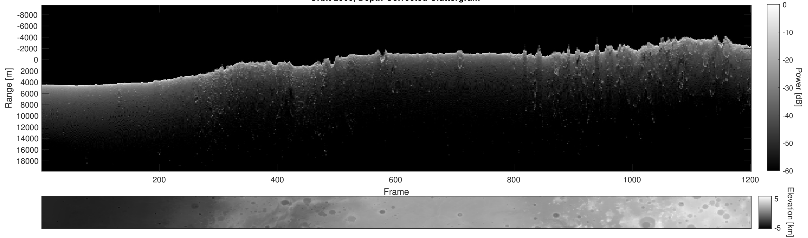
Orbit 2966, Depth-Corrected Cluttergram
