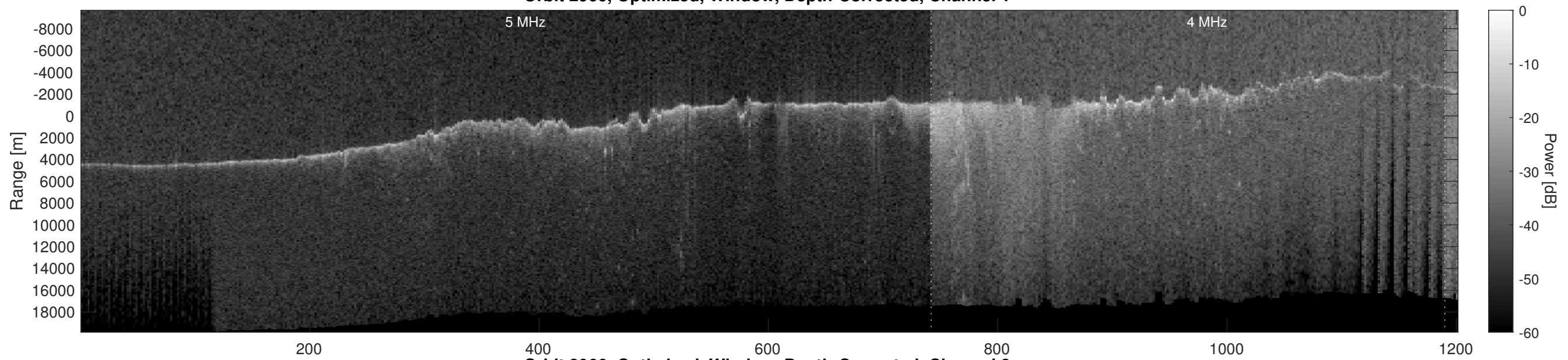
Orbit 2966, Optimized, Window, Depth-Corrected, Channel 2
