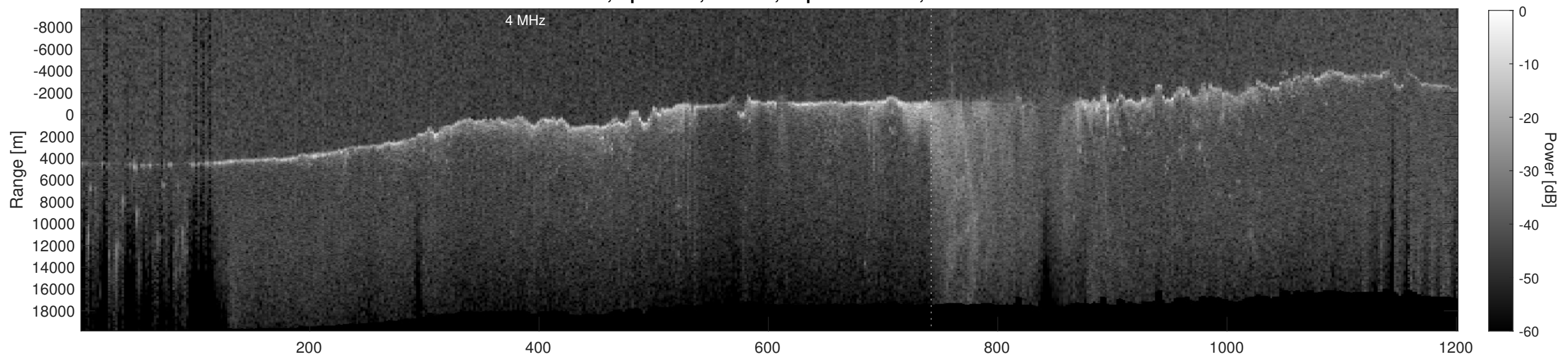
Orbit 2966, Depth-Corrected Cluttergram
