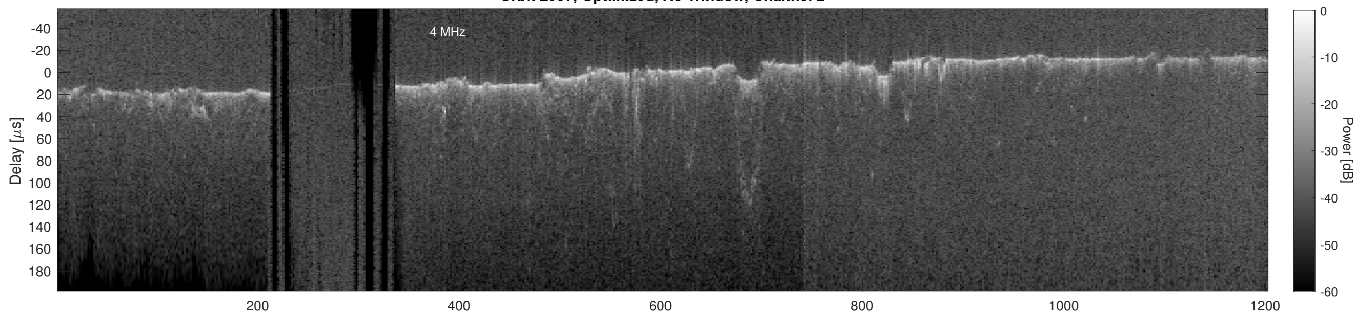
Orbit 2967, Cluttergram
