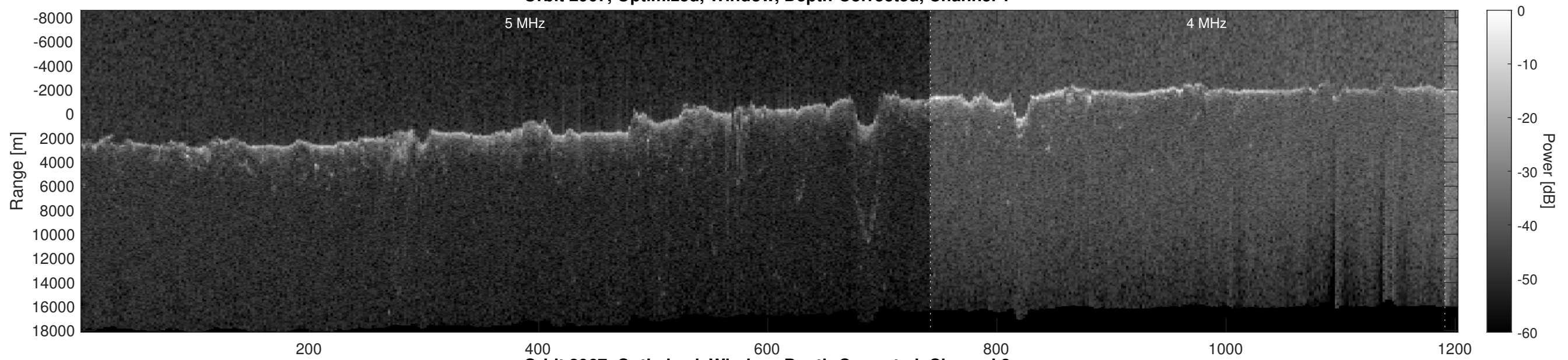
Orbit 2967, Optimized, Window, Depth-Corrected, Channel 2
