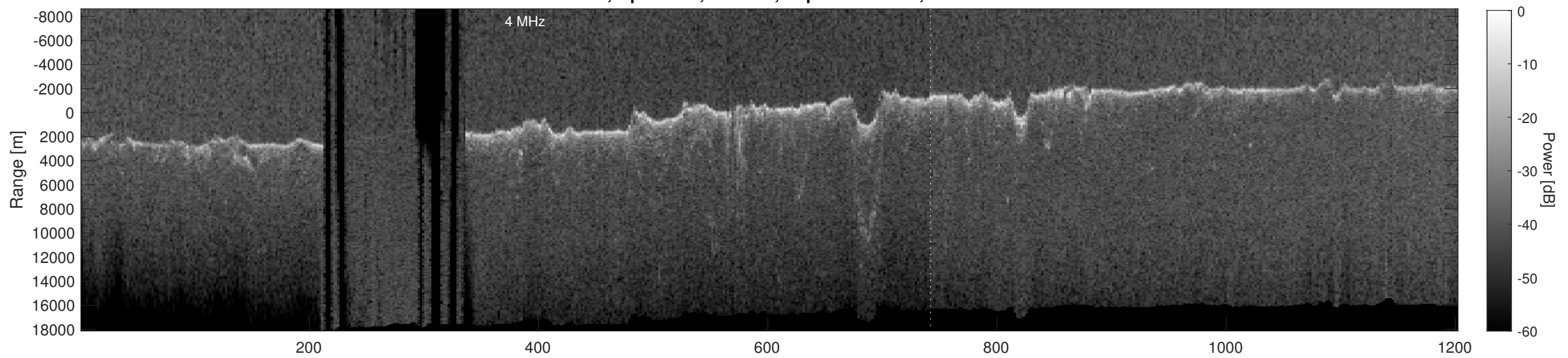
Orbit 2967, Depth-Corrected Cluttergram
