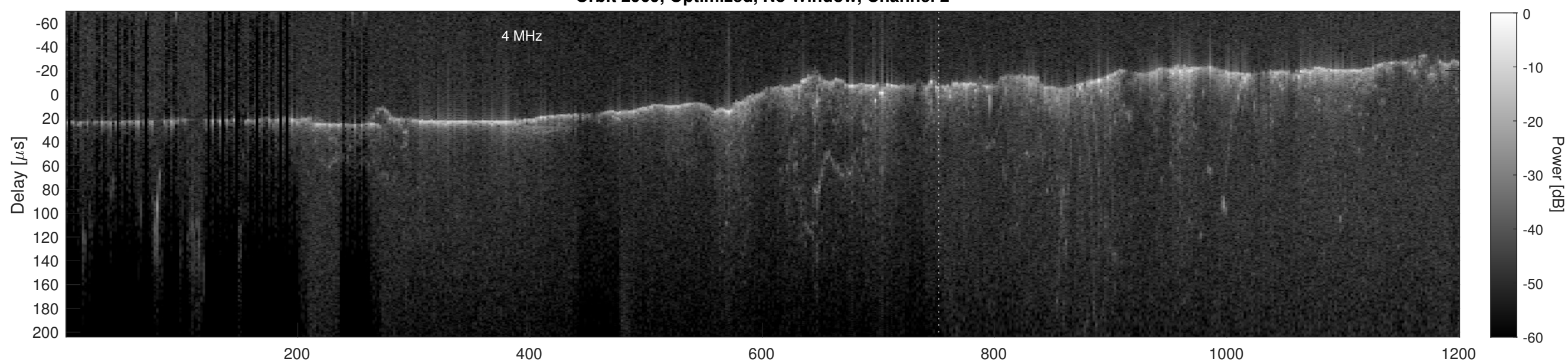
Orbit 2969, Cluttergram
