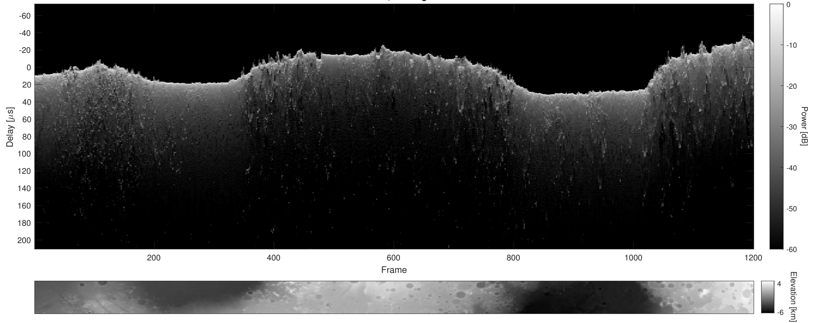
Orbit 2970, Cluttergram
