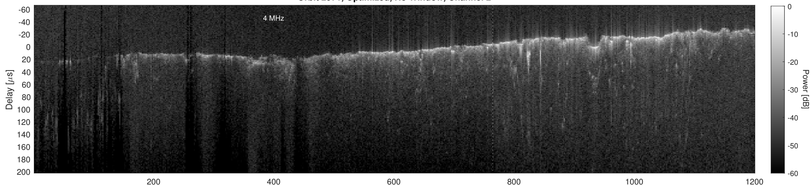
Orbit 2971, Cluttergram
