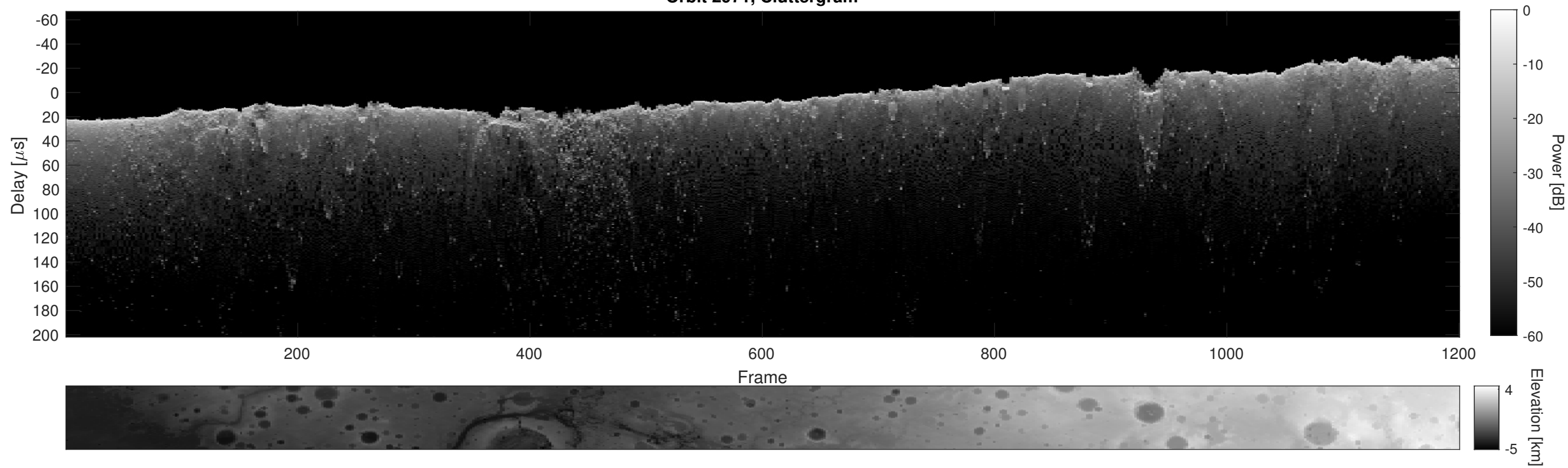
Orbit 2971, Cluttergram
