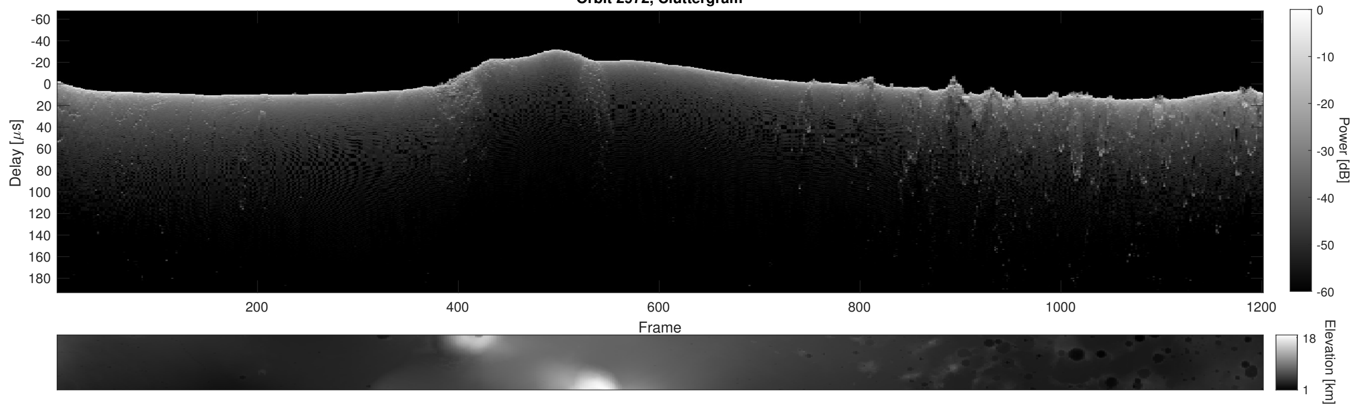
Orbit 2972, Cluttergram
