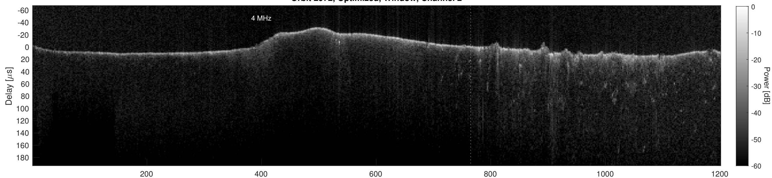
Orbit 2972, Cluttergram
