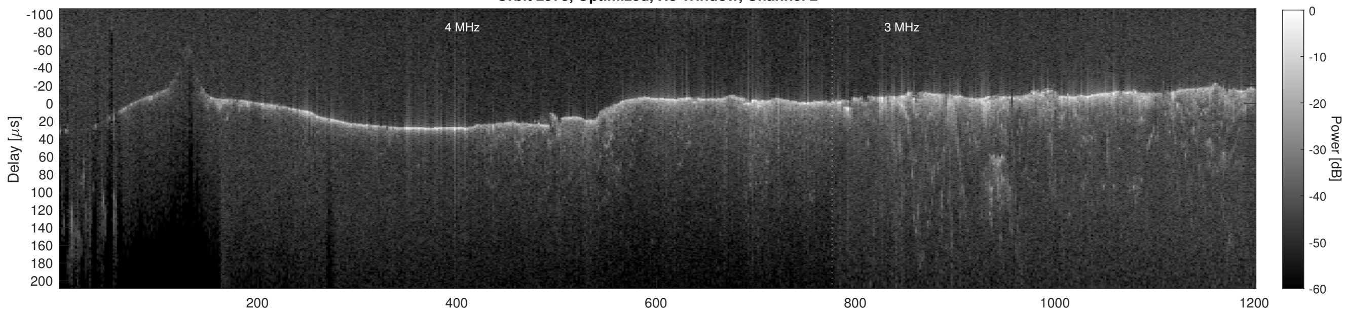
Orbit 2973, Cluttergram
