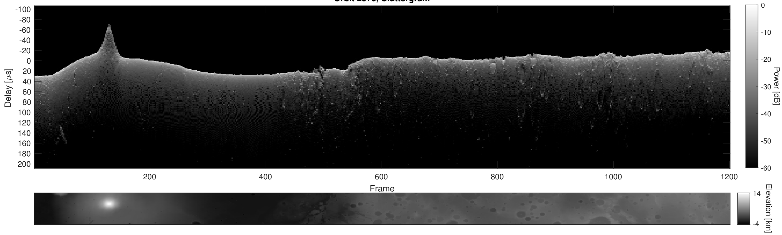
Orbit 2973, Cluttergram
