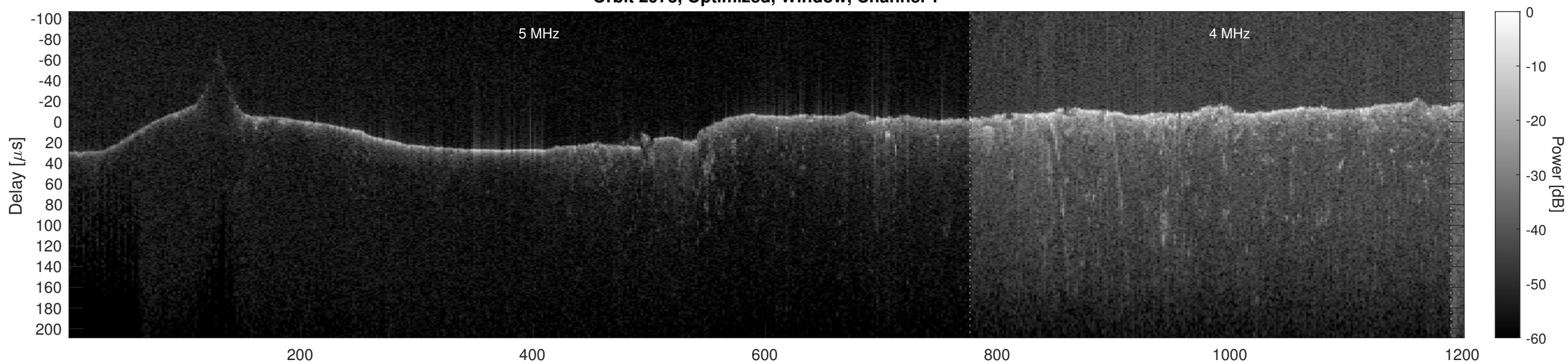
Orbit 2973, Optimized, Window, Channel 2
