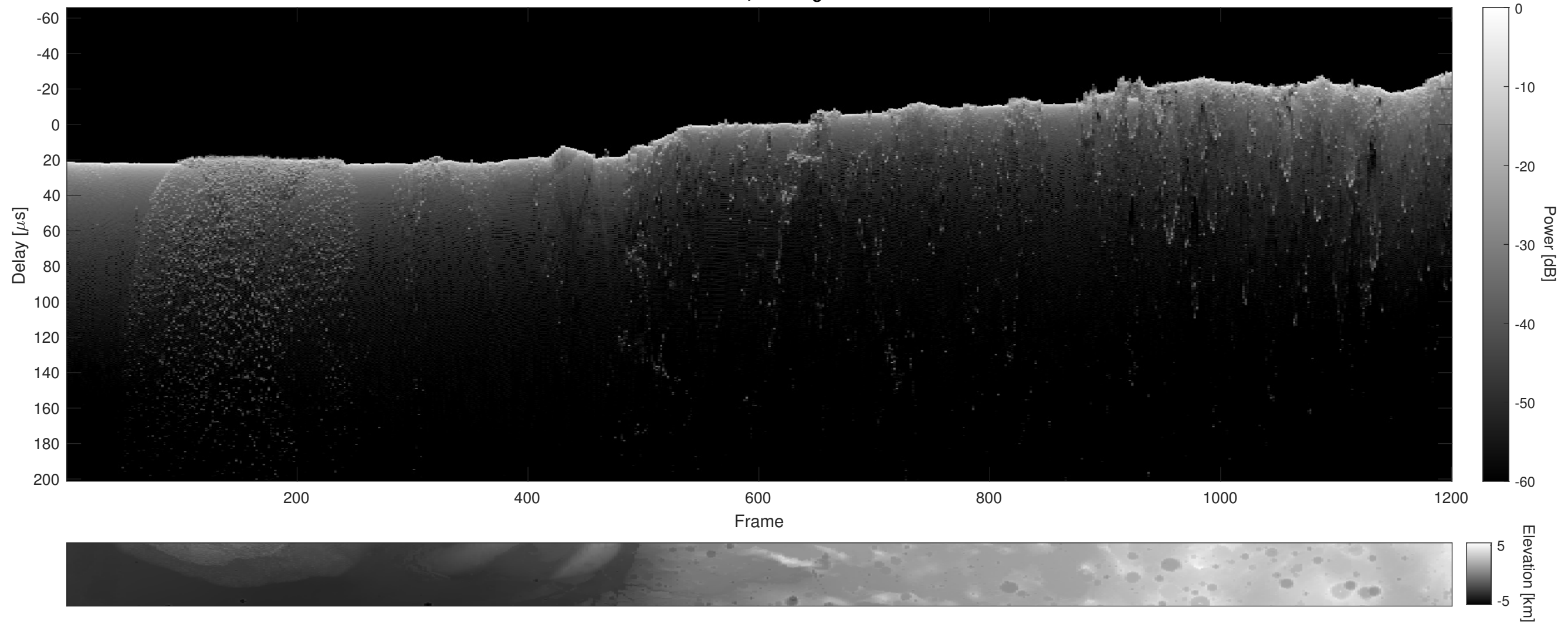
Orbit 2976, Cluttergram
