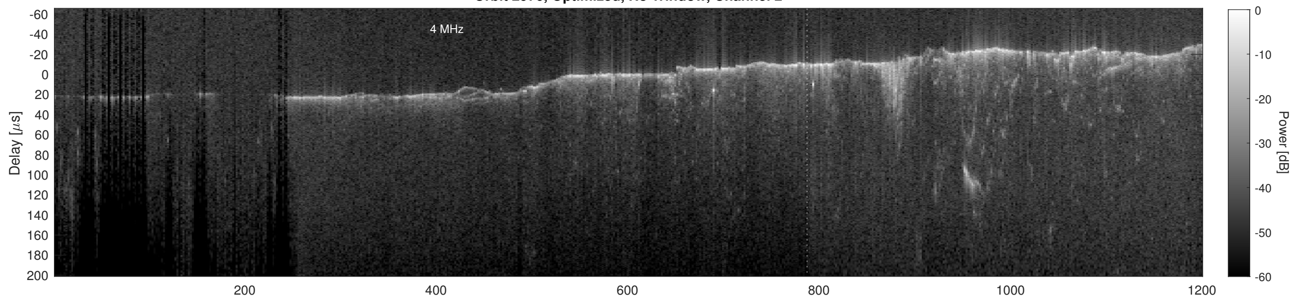
Orbit 2976, Cluttergram
