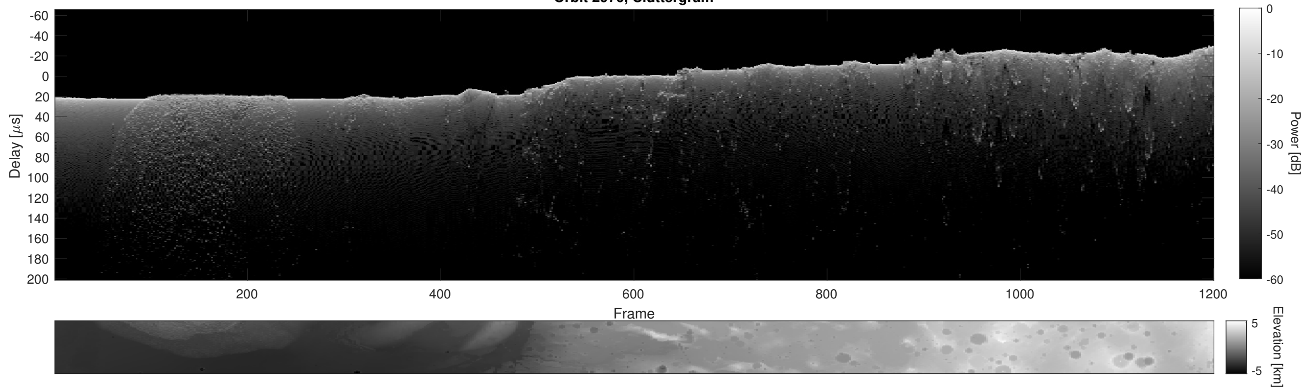
Orbit 2976, Cluttergram
