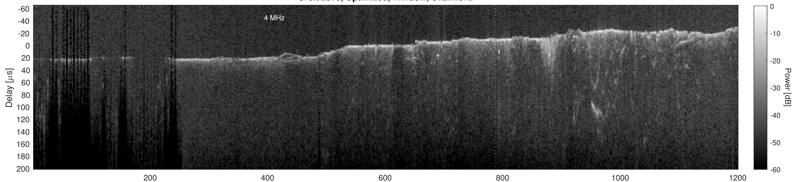
Orbit 2976, Cluttergram
