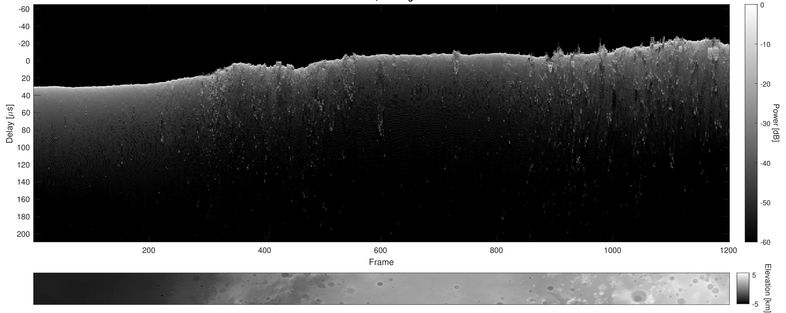
Orbit 2977, Cluttergram
