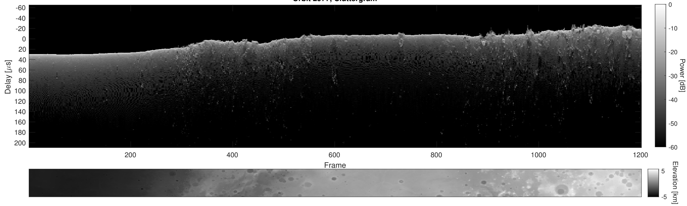
Orbit 2977, Cluttergram
