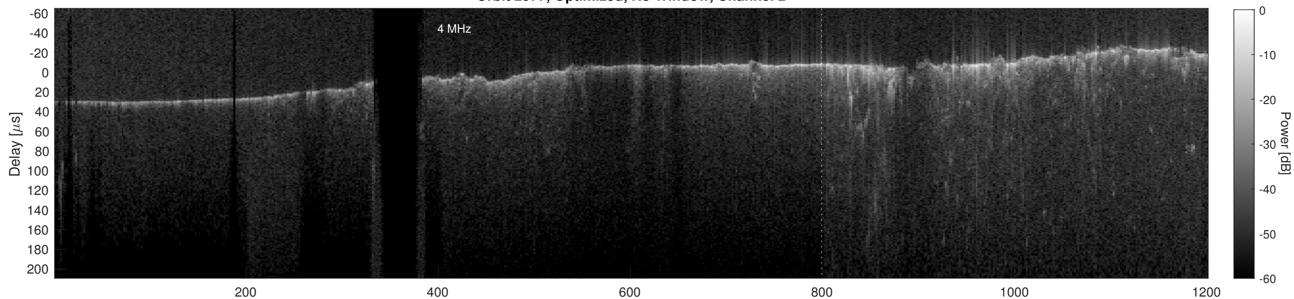
Orbit 2977, Cluttergram
